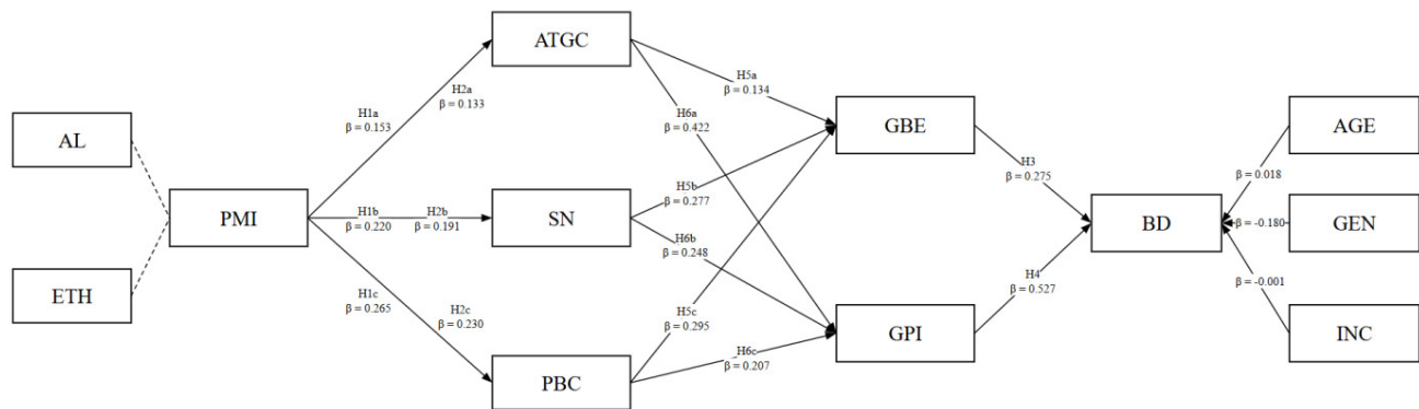
Figure 2. Pathway diagram of the research model
